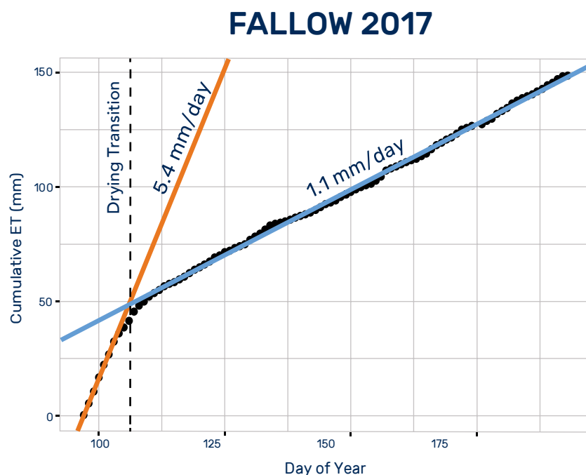
Figure 15. Measured cumulative evaporation from a summer fallow site in the BWD. The initial evaporation rate was 5.4 mm/day (0.2 in/day) for the first 10 days (before vertical dashed line), then decreased to a constant 1.1 mm/day (0.04 in/day) thereafter.
